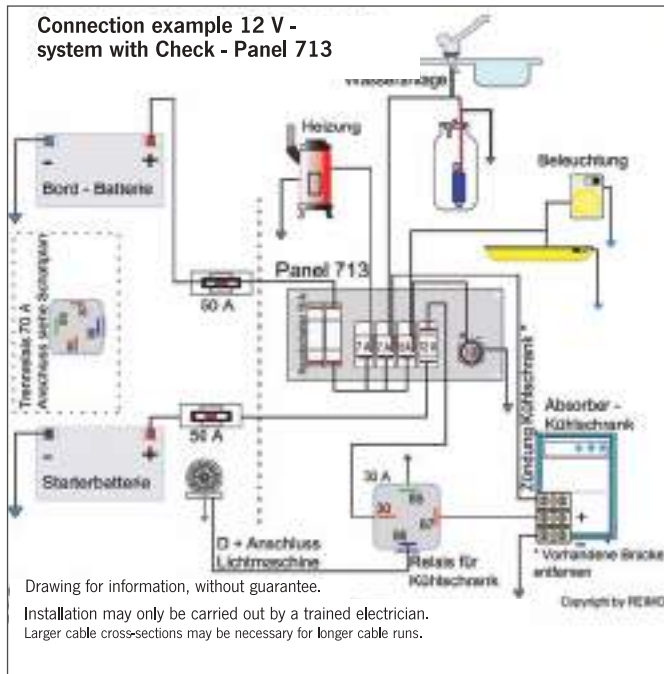
Connection example of a CEE system
